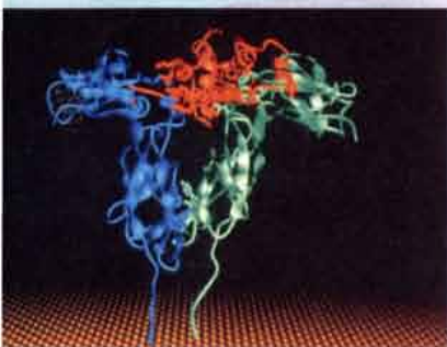
X-ray crystallographic analysis of human growth hormone protein
