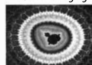
Fractals
