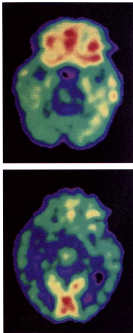
FUNCTIONAL DEFICIENCY is evident in positron emission tomographic scans made while the subjects were taking a test of vigilance. The test enhances prefrontal cortex metabolism in the normal volunteer ( top ) but not in the schizophrenic patient ( bottom ). The data were provided by Monte S. Buchsbaum of the University of California at Irvine.
