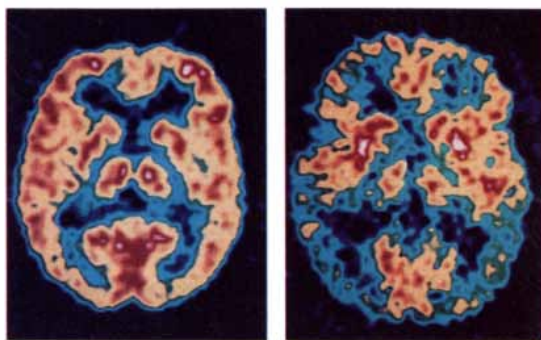
PET SCANS OF BRAINS from a healthy aged adult (left) and a patient with Alzheimer's disease (right) differ markedly. The excess of dark shading in the second image shows that brain activity is impaired.
