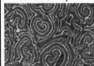
Chaos/Artificial Life
