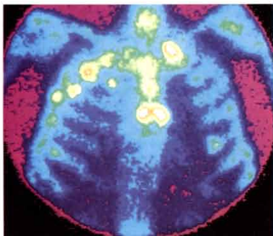
Secondary tumors, or metastases, appear as small colored "hotspots" against the background blue of a cancer patient's chest in this radioisotope scan.
