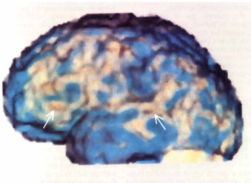
LANGUAGE ACTIVITY is visible in this positron emission tomographic (PET) scan of a normal individual performing a naming task. The PET image has been projected onto a three-dimensional magnetic resonance imaging (MRI) reconstruction of the same individual's brain. There are many areas of increased activity in the left hemisphere, including the motor cortex and the anterior and posterior language sectors (arrows). The image was produced by the University of Iowa's Department of Neurology, PET Facility and Image Analysis Facility.
